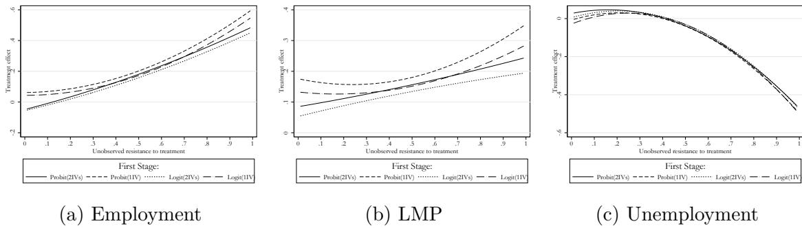
Figure A.10: MTE: Alternative First Stage Estimators
