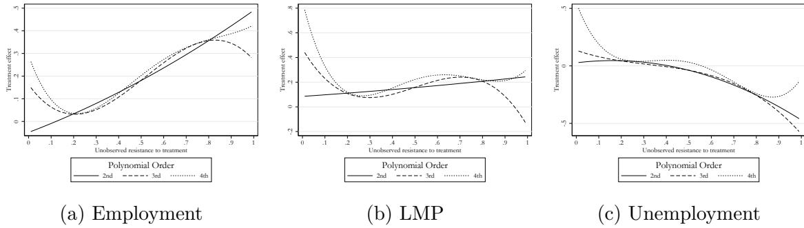
Figure A.11: MTE: Alternative Polynomials
