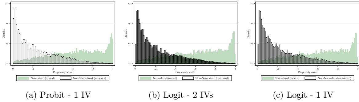
Figure A.9: Common Support: Robustness Checks
